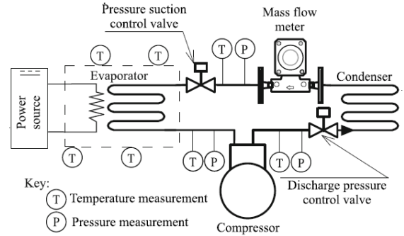
Figure 1: Simplified schematic of the test rig.
